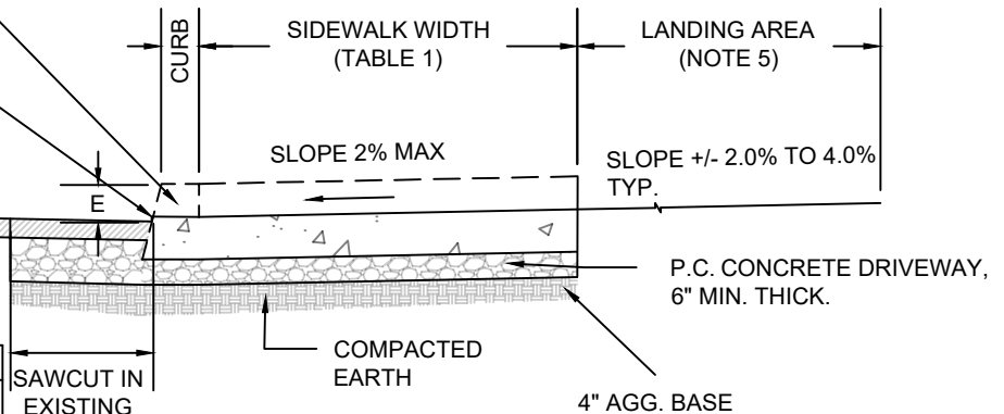
TYPICAL PLAN AND PROFILE VIEW DRIVEWAY APPROACH, CURB-TIGHT, FULLY LOWERED (ALTERNATE C)
